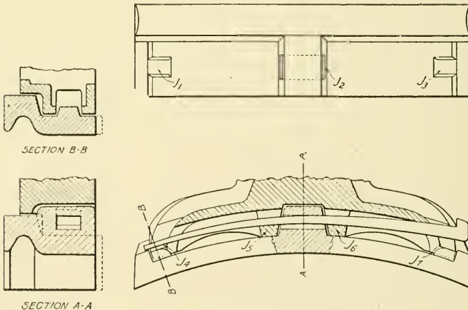
Fig. 21. American Electric Railway Engineering Association Standard Brake Shoe
